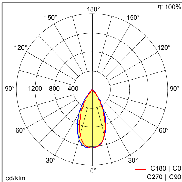
TE_LILY_LED_SPOT_IP44_60_68_850_940.idt
