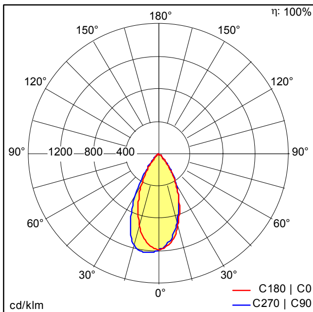
TE_LILY_LED_SPOT_IP44_60_68_600_927.idt
