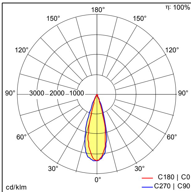
TE_LILY_LED_SPOT_IP44_24_68_600_930.idt
