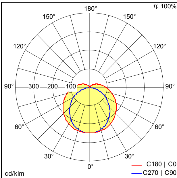
TE_POPPY_LED_1500_4500_840.ltd
