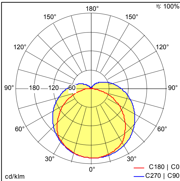
TE_POPPY_LED_1800_8500_840_E3e.ltd
