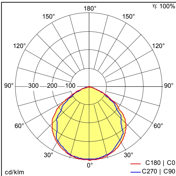
TE_LEONIE_LED_FL_IP65_50W_830.ltd
