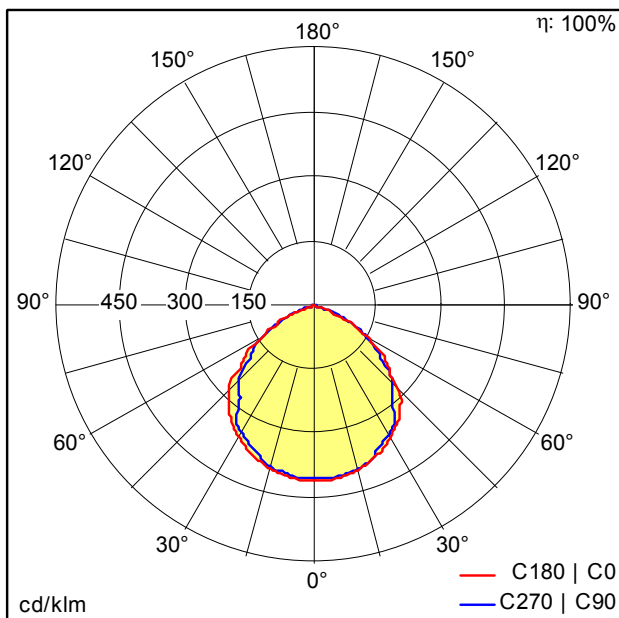
TE_LEONIE_LED_FL_IP65_50W_830.idt
