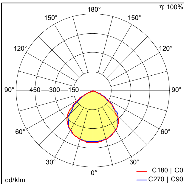
TE_LEONIE_LED_FL_IP65_30W_830.idt
