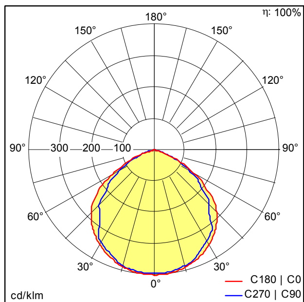
TE_LEONIE_LED_FL_IP65_50W_840.idt
