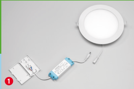
1 Unplug the connector between the Zoe slim downlight and the driver.
